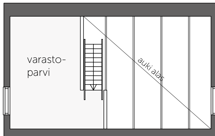
NALLE 30A, B, C, D PARVI
